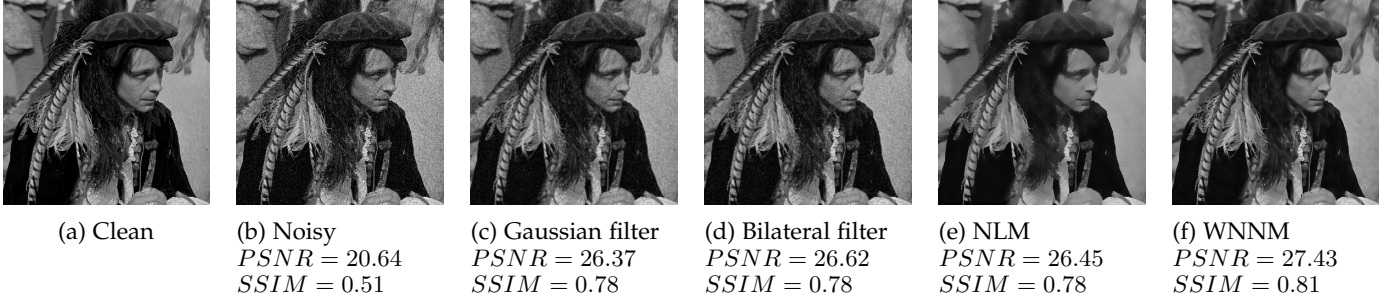
Fig. 4: Clean, noisy (zero mean Gaussian noise with \sigma = 0.1 ), and denoised images produced using the different methods.
